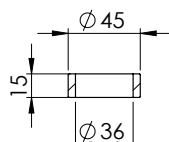
S.S. Bushing P/N 207133
