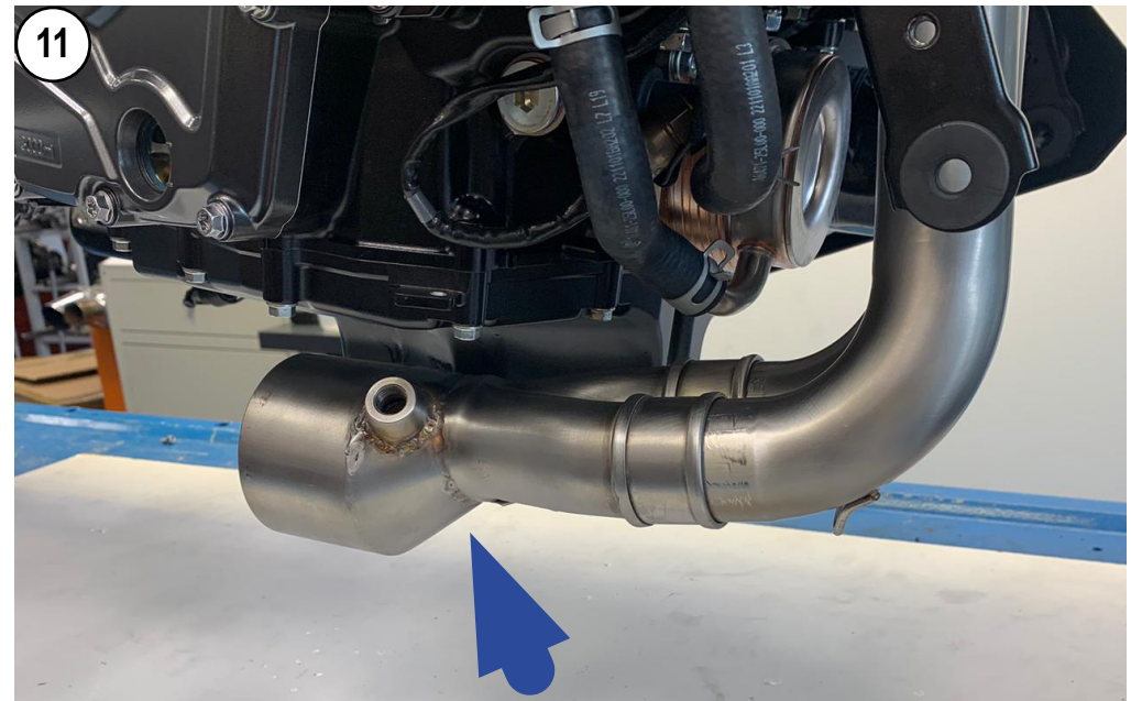
11 SLIDE IN THE SECONDARY PIPE
