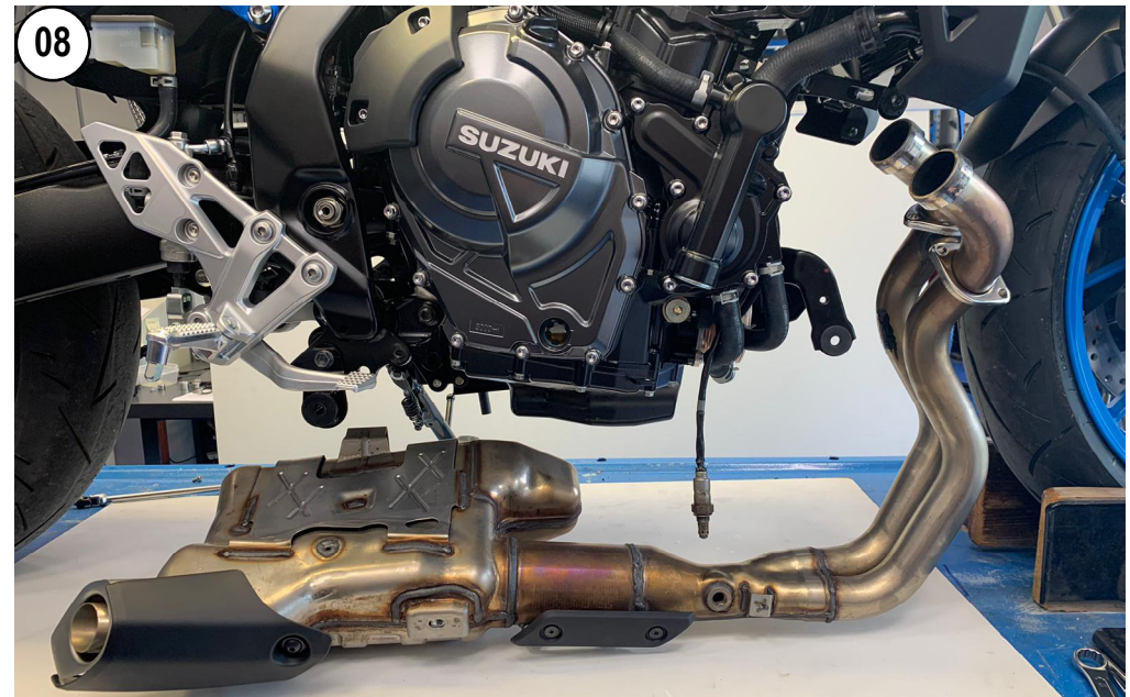
REMOVE THE ENTIRE ORIGINAL EXHAUST SYSTEM
