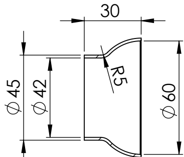
S.s. bushing cod.207042
