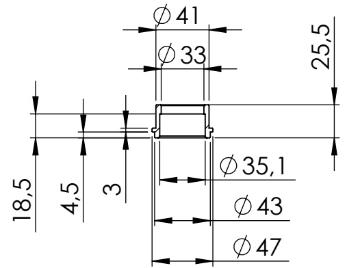
S.S. Bushing P/N 204833
